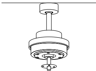
Traditional assembly
